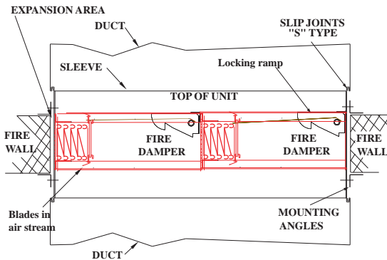
HORIZONTAL INSTALLATION
