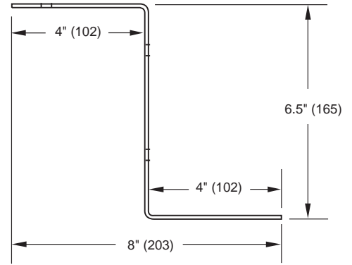
Figure 3: Shelf Bracket
