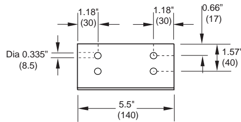
Figure 4: Support Angle
